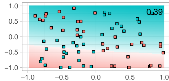
naive bayes
