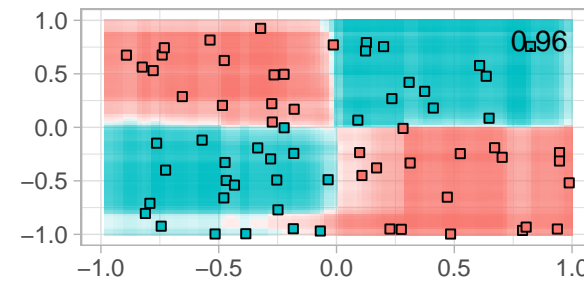
random forest
