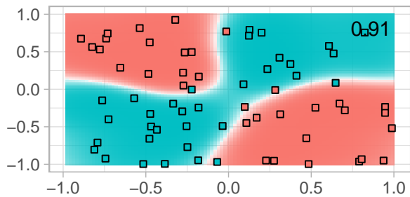
rbf svm
